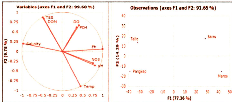
Figure 8. Principal component analysis of physico-chemical parameters from the study sites.
