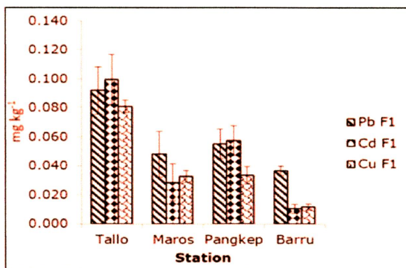
Figure 5. Labile fraction (F1) of Pb, Cd and Cu concentrations measured in the sediments of west coast, South Sulawesi.
