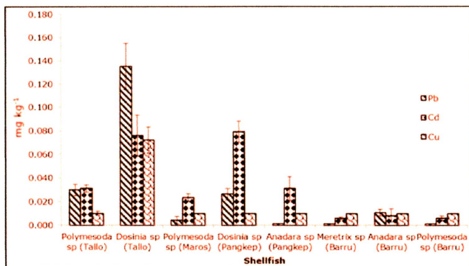
Figure 6. Content of metals ( \text{mg kg}^{-1} dry weight); mean \pm standard deviation.
