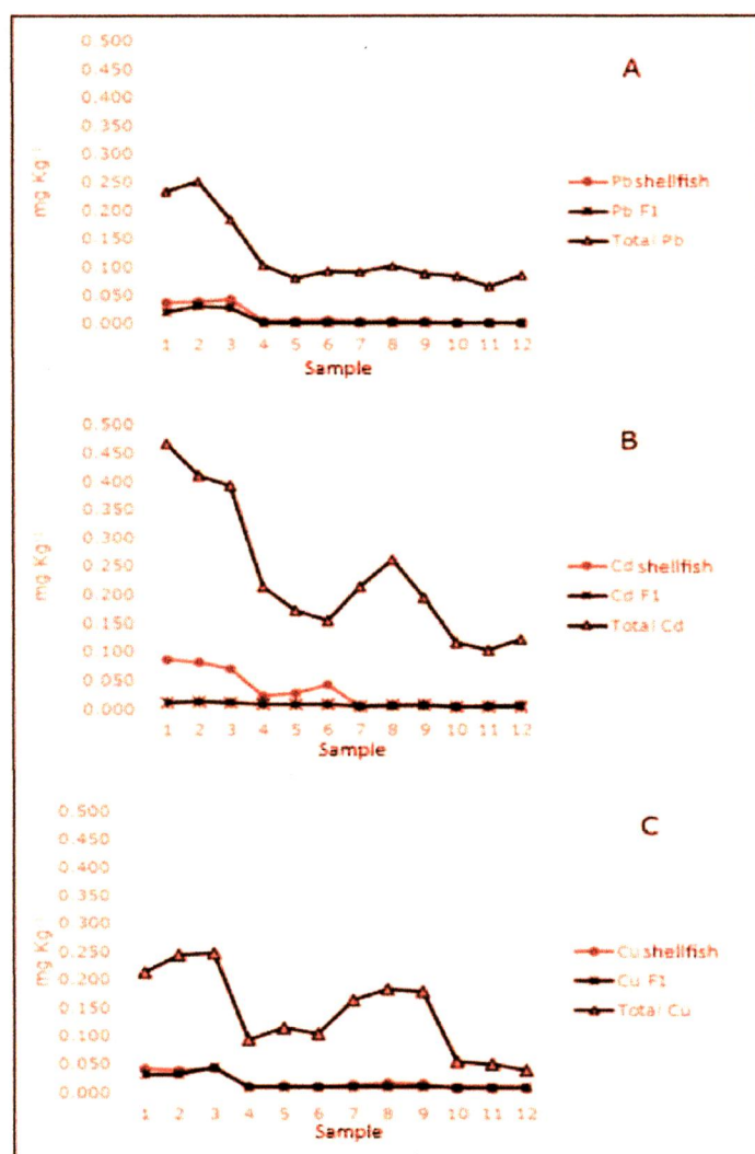
Figure 3 Relationship between concentrations of metals in shellfish tissue with labile fractions and total metals in the estuary sediments of the west coast of South Sulawesi. A - Pb; B - Cd; C - Cu.
