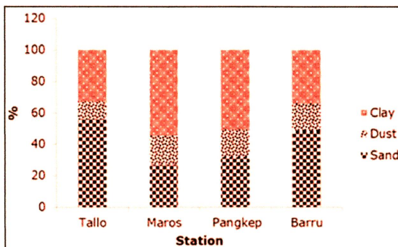
Figure 2. Sediment texture in west coastal South Sulawesi sediments.
